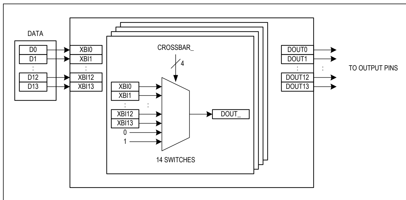
Figure 17. Crosspoint-Switch Dataflow
