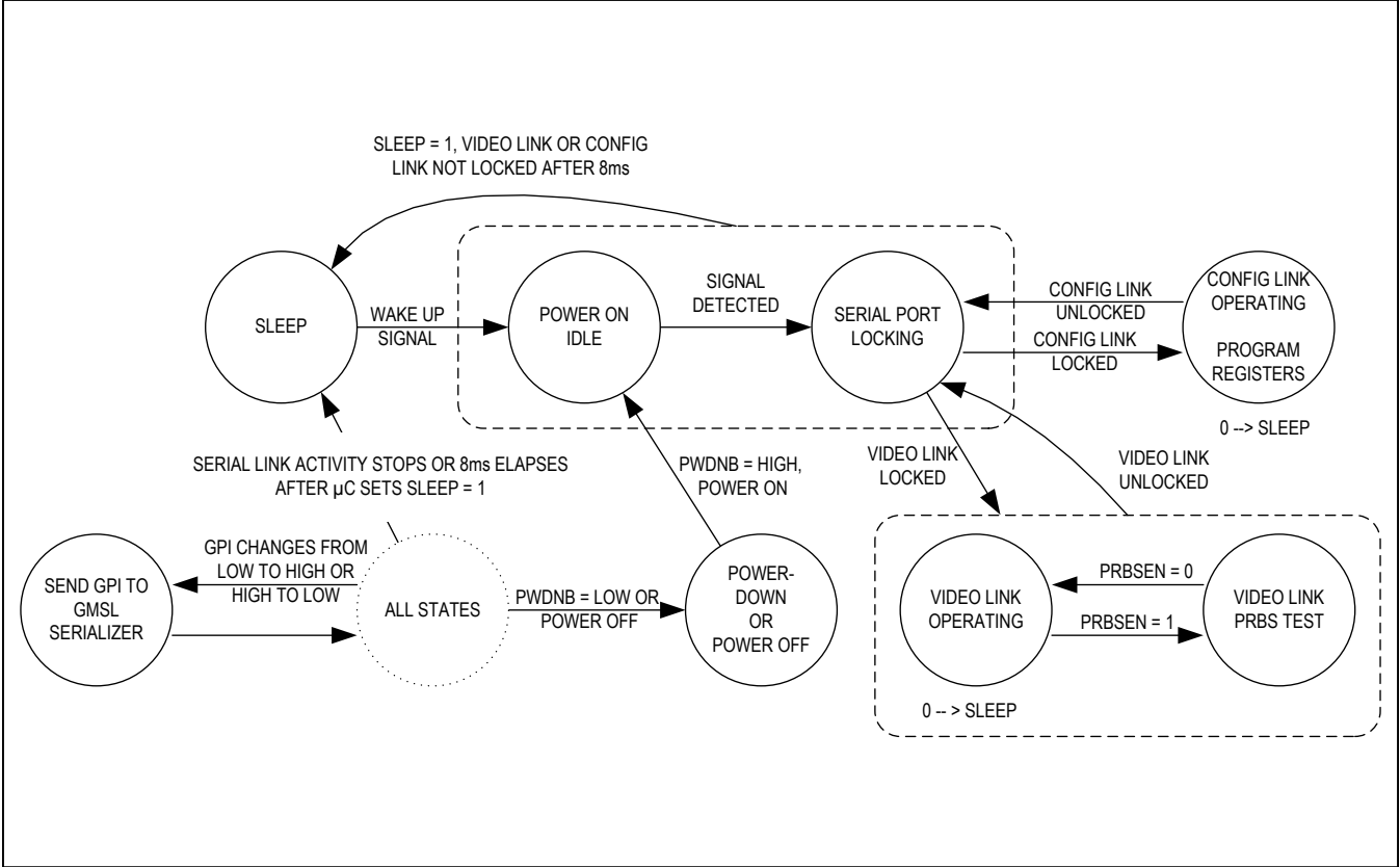
Figure 18. State Diagram
