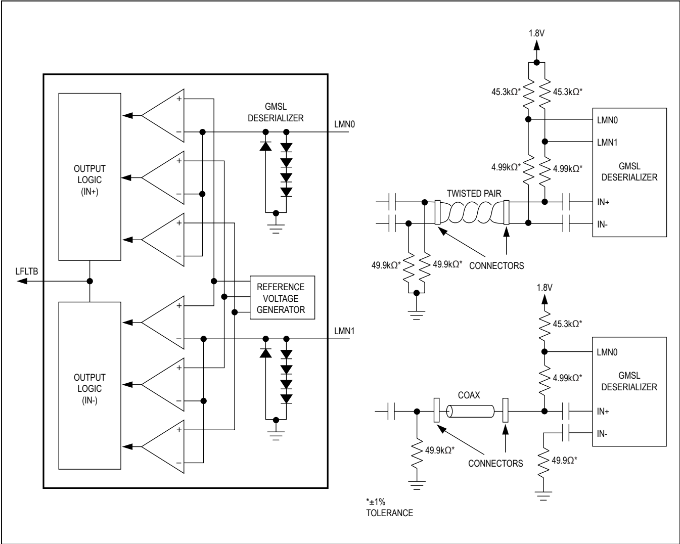
Figure 4. Line Fault
