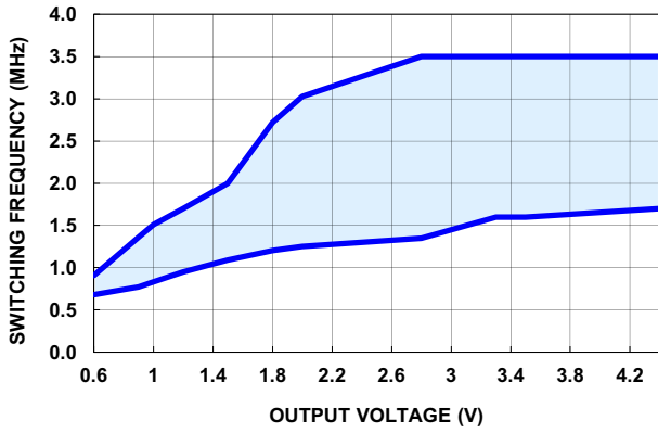
FIGURE 6. OPERATION REGION V IN = 5.0V
