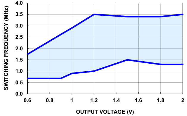
FIGURE 9. OPERATION REGION V IN = 2.6V
