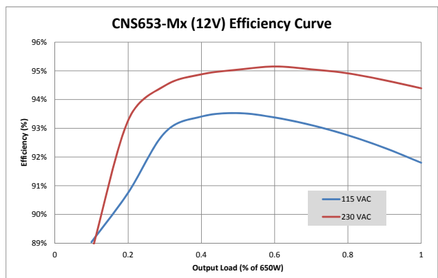
Figure 3. Typical Efficiency for 12 V Output
