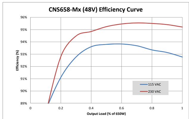
Figure 5. Typical Efficiency for 48 V Output
