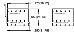
VCH CONNECTOR HOUSING
