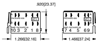
VC1 CONNECTOR HOUSING
