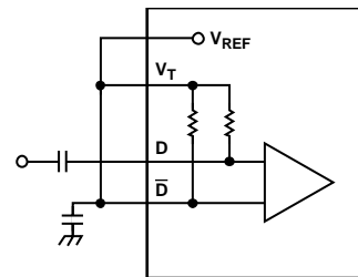
CONNECT V_T , V_{REF} , AND \bar{D} . PLACE A BYPASS CAPACITOR FROM V_T TO GROUND. ALTERNATIVELY, V_T , V_{REF} , AND D CAN BE CONNECTED, GIVING A CLEANER LAYOUT AND A 180^\circ PHASE SHIFT. 06318-030
