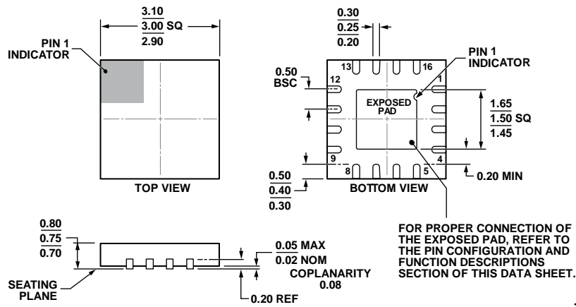
Figure 31. 16-Lead Lead Frame Chip Scale Package [LFCSP] 3 mm x 3 mm Body and 0.75 mm Package Height (CP-16-27) Dimensions shown in millimeters
