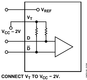
CONNECT V_T TO V_{CC} - 2V . 06318-028
