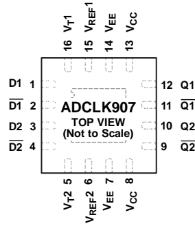
Figure 5. ADCLK907 Pin Configuration
