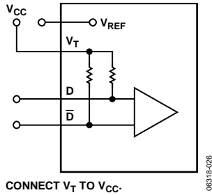
CONNECT V_T TO V_{CC} . 06318-026
