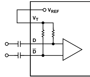
CONNECT V_T TO V_{REF} . NOTES 1. PLACING A BYPASS CAPACITOR FROM V_T TO GROUND CAN IMPROVE THE NOISE PERFORMANCE. 06318-029
