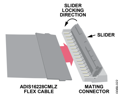
Figure 26. Mating Connector Detail
