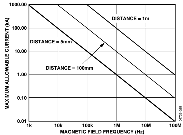
Figure 28. Maximum Allowable Current for Various Current-to- ADM2483 Spacings
