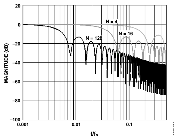
Figure 22. Frequency Response—Moving Average Filter
