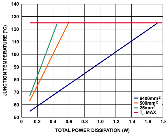
Figure 72. LFCSP, T_A = 50^\circ\text{C}
