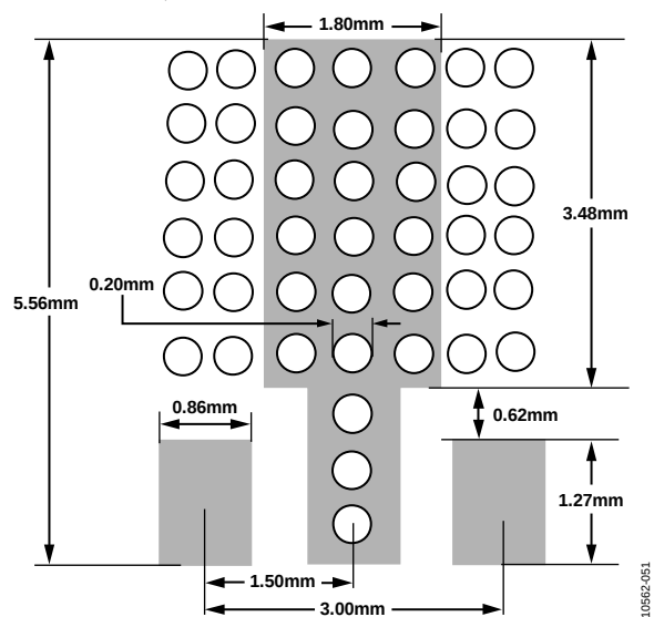
Figure 35. Recommended Land Pattern
