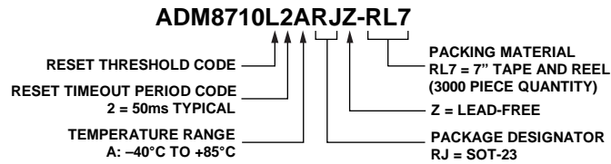
Figure 16. ADM8710 Ordering Code Structure
