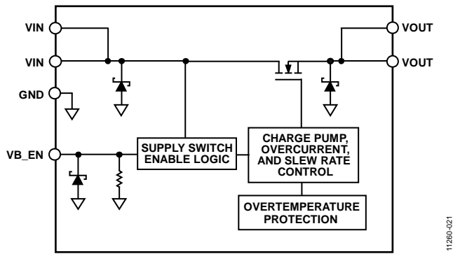
Figure 21. Functional Block Diagram
