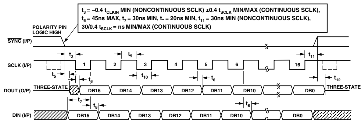
Figure 35. SPI/QSPI Mode 2 Timing Diagram for Read/Write Operation with \overline{\text{SYNC}} Input Edge Triggered (SM1 = SM2 = 0)
