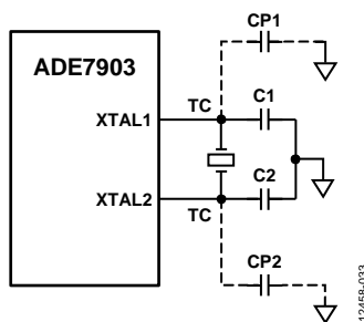
Figure 33. Crystal Circuitry
