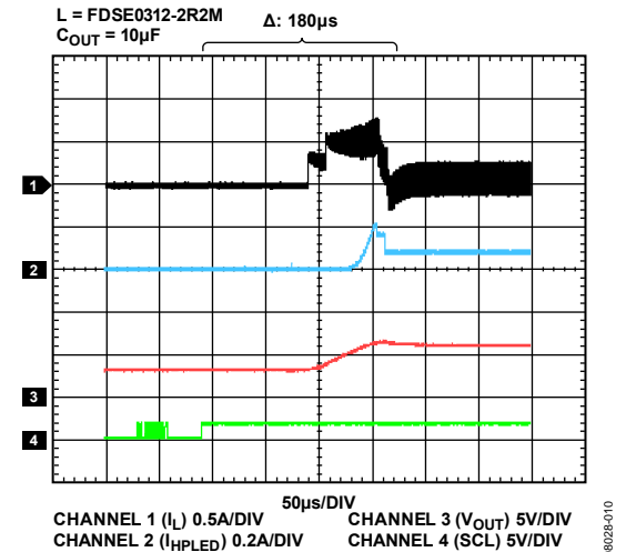
Figure 10. Startup, Two LEDs Torch Mode, I_{LED} = 40 mA, V_{IN} = 3.6 V
