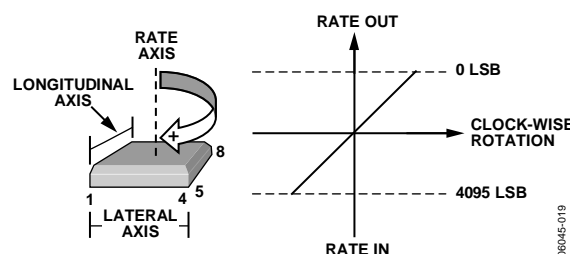
Figure 20. Rate Signal Increases with Clockwise Rotation
