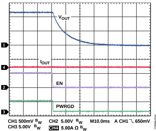
Figure 36. Channel 1/Channel 2 Shutdown with Active Output Discharge, V_{IN} = 12\text{ V} , V_{OUT} = 1.2\text{ V} , f_{SW} = 600\text{ kHz} , L = 1\text{ μH} , C_{OUT} = 47\text{ μF} \times 2
