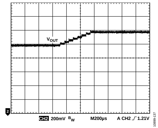
Figure 39. Channel 1 Dynamic Voltage Scaling (DVS) from 1.1 V to 1.3 V, 62.5\text{ μs} Interval, V_{IN} = 12\text{ V} , I_{OUT} = 4\text{ A} , f_{SW} = 600\text{ kHz} , L = 1\text{ μH} , C_{OUT} = 47\text{ μF} \times 2
