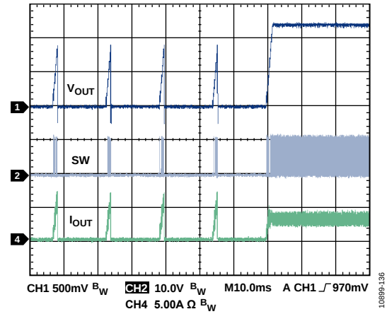
Figure 38. Short-Circuit Protection Recovery, V_{IN} = 12\text{ V} , V_{OUT} = 1.2\text{ V} , f_{SW} = 600\text{ kHz} , L = 1\text{ μH} , C_{OUT} = 47\text{ μF} \times 2
