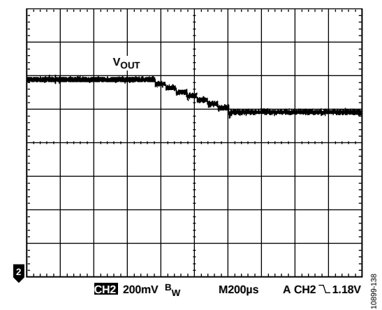
Figure 40. Channel 1 Dynamic Voltage Scaling (DVS) from 1.3 V to 1.1 V, 62.5\text{ μs} Interval, V_{IN} = 12\text{ V} , I_{OUT} = 4\text{ A} , f_{SW} = 600\text{ kHz} , L = 1\text{ μH} , C_{OUT} = 47\text{ μF} \times 2
