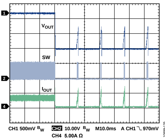
Figure 37. Short-Circuit Protection Entry, V_{IN} = 12\text{ V} , V_{OUT} = 1.2\text{ V} , f_{SW} = 600\text{ kHz} , L = 1\text{ μH} , C_{OUT} = 47\text{ μF} \times 2
