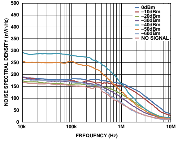
Figure 31. Noise Spectral Density, C_{FLT} = Open, 25^\circ\text{C}
