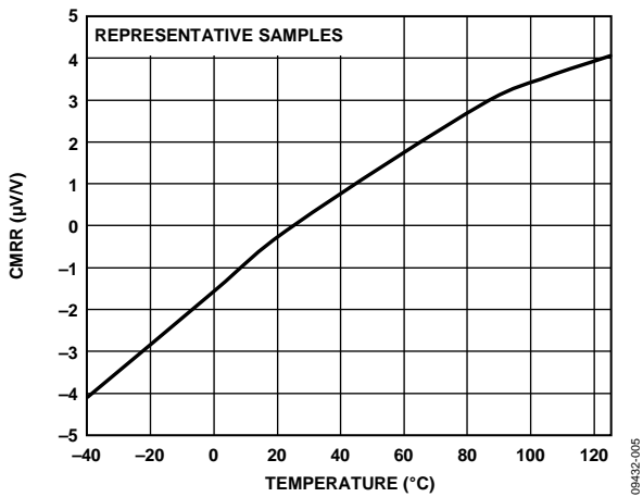
Figure 6. CMRR vs. Temperature (G = 0.8)
