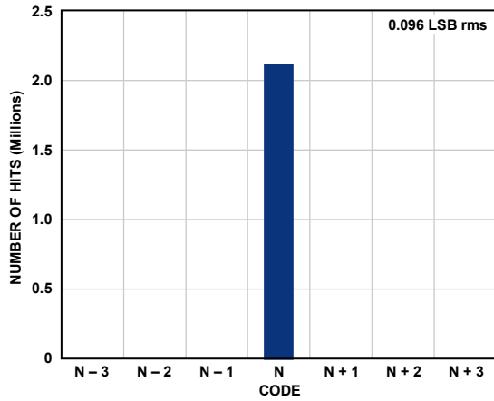
Figure 39. Input-Referred Noise Histogram, AD9212-65
