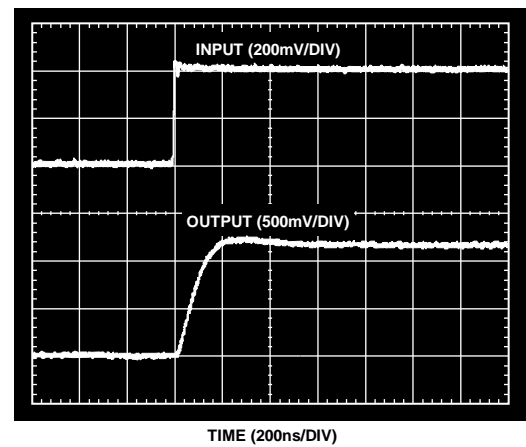
Figure 8. Rise Time
