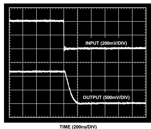
Figure 9. Fall Time
