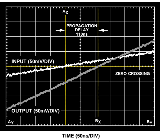
Figure 20. Propagation Delay (Rising)
