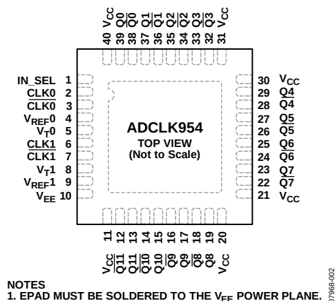
Figure 2. Pin Configuration
