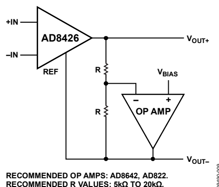
Figure 70. Differential Output Using an Op Amp
