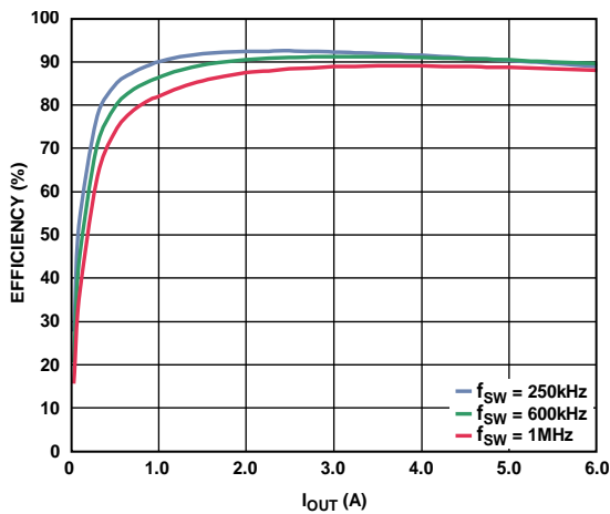
Figure 6. Channel 1/Channel 2 Efficiency Curve, V_{IN} = 12\text{ V} , V_{OUT} = 3.3\text{ V} , MOSFET = SI4204DY, FPWM Mode
