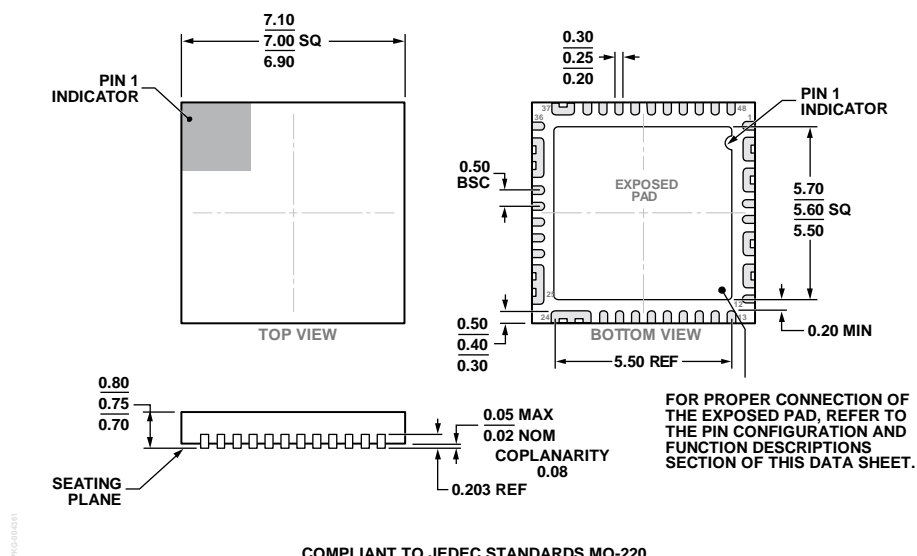
Figure 45. 48-Lead Lead Frame Chip Scale Package [LFCSP_WQ] 7 mm x 7 mm Body, Very Very Thin Quad with Fused Leads (CP-48-16) Dimensions shown in millimeters
