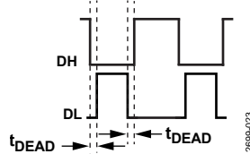
Figure 25. Dead Time ( t_{\text{DEAD}} ) Between DH and DL Transitions
