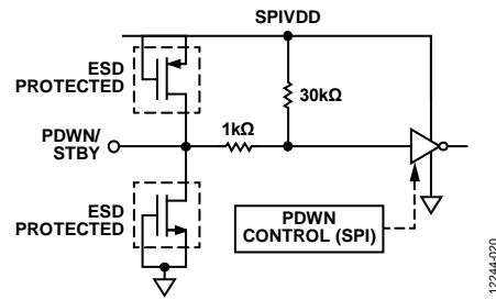
Figure 61. PDWN/STBY Input
