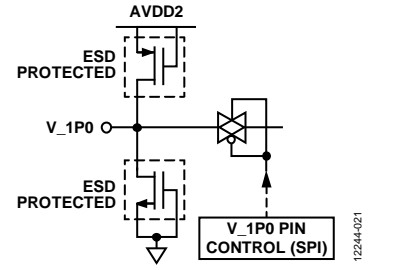
Figure 62. V_1P0 Input
