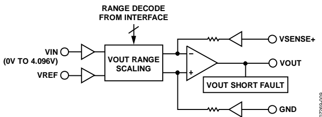
Figure 53. Voltage Output
