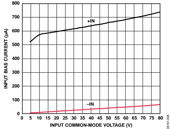
Figure 8. Input Bias Current vs. Input Common-Mode Voltage ( V_{DIFF} = 5\text{ mV} )
