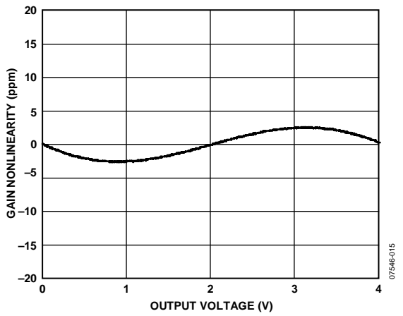
Figure 16. Gain Nonlinearity, R_L = 600\ \Omega , 2 k \Omega , 10 k \Omega
