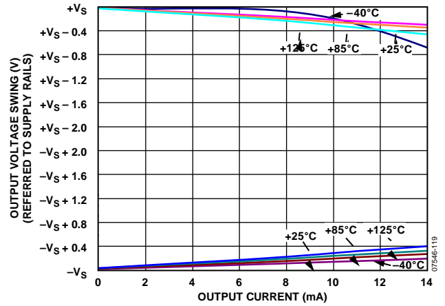
Figure 20. Output Voltage Swing vs. Output Current, V_S = 5\text{ V}
