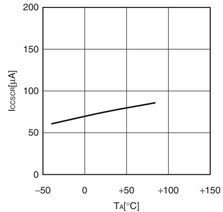
I_{CCSCR} - T_A V_{CC} = 5.5\text{ V} , F_{MPL} = 50\text{ kHz} (divided by 2) Sub-CR clock mode
