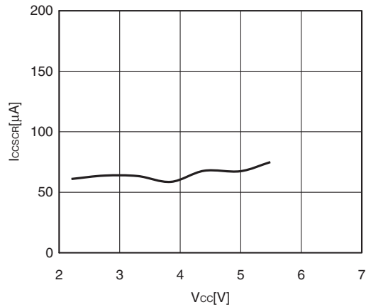
I_{CCSCR} - V_{CC} T_A = +25^\circ\text{C} , F_{MPL} = 50\text{ kHz} (divided by 2) Sub-CR clock mode
