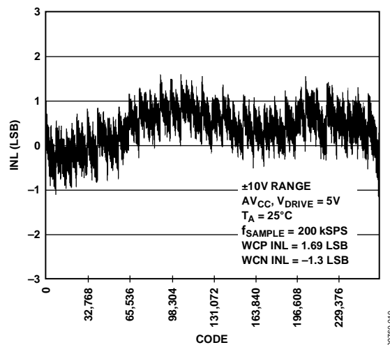
Figure 11. Typical INL, ±10 V Range
