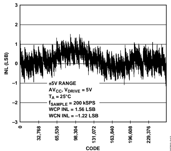
Figure 13. Typical INL, ±5 V Range
