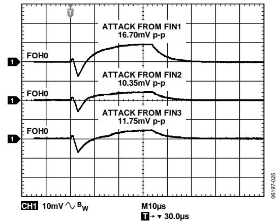
Figure 33. AC Crosstalk at FOH0 in FI Mode from FIN DAC of Each Other PMU (Full-Scale Transition), MI Gain = 10, MEASOUT Gain = 1, \pm 2 mA Range, C_{LOAD} = 200 pF
