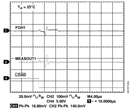
Figure 32. AC Crosstalk, FVMI Mode, PMU 1, Full-Scale Transition on One CPH DAC, MI Gain = 10, MEASOUT Gain = 1, \pm 2 mA Range, C_{LOAD} = 200 pF
