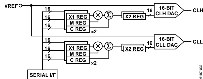
Figure 53. Clamp Registers
