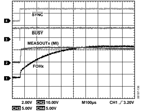
Figure 44. FV Settling, 0 V to 5 V, \pm 5 \mu\text{A} Range, C_{\text{LOAD}} = 220 \text{ pF} , \text{CCOMP}_x = 100 \text{ pF} , R_{\text{LOAD}} = 1 \text{ M}\Omega
