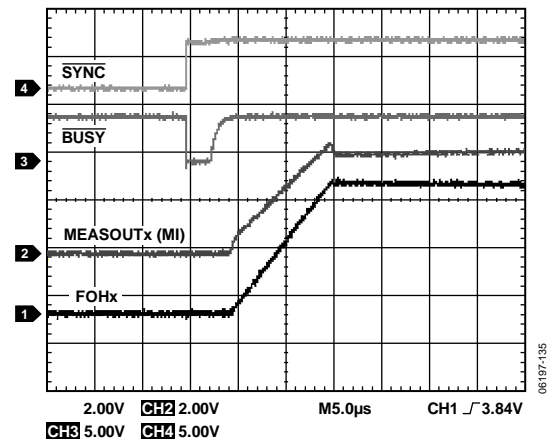
Figure 43. FV Settling, 0 V to 5 V, \pm 2 \text{ mA} Range, C_{\text{LOAD}} = 220 \text{ pF} , \text{CCOMP}_x = 100 \text{ pF} , R_{\text{LOAD}} = 5.6 \text{ k}\Omega
