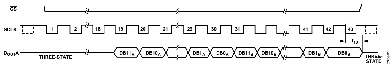
Figure 34. Reading Data from Both ADCs on One D_{OUT} Line with 43 SCLKs
