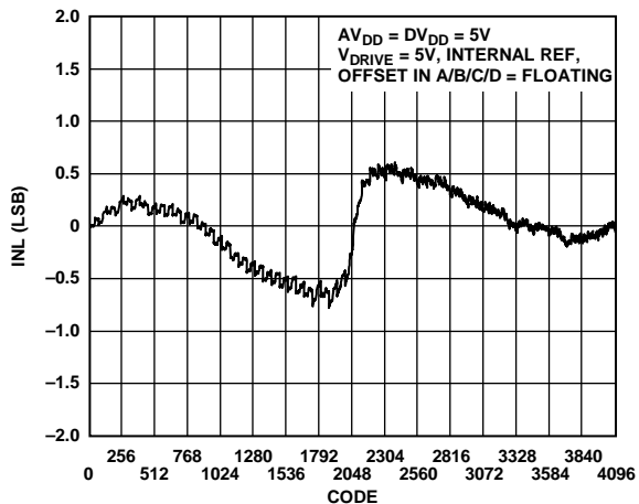
Figure 20. DAC INL
