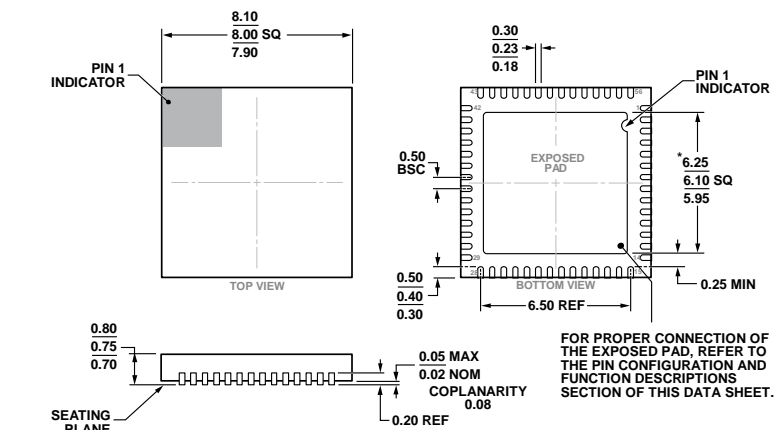
Figure 63. 56-Lead Lead Frame Chip Scale Package [LFCSP] 8 mm × 8 mm body and 0.75mm Package Height (CP-56-11)
