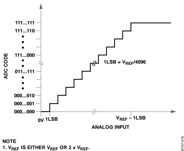
Figure 35. Single-Ended Transfer Characteristic
