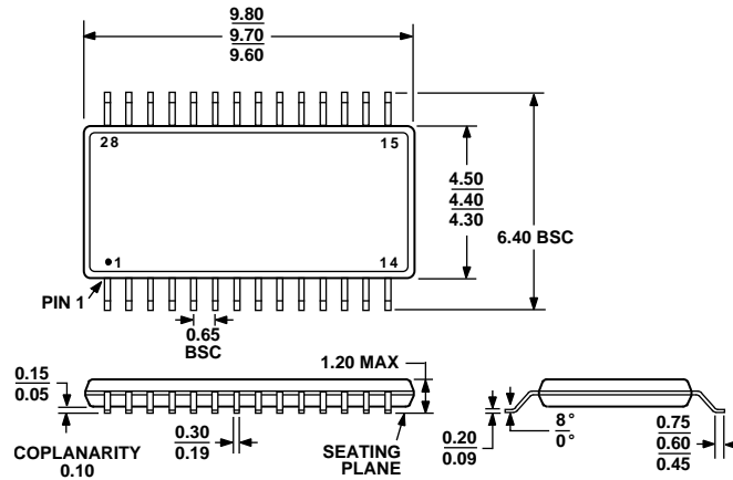
Figure 54. 28-Lead Thin Shrink Small Outline [TSSOP] (RU-28)
