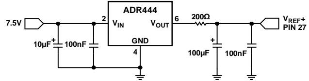
Figure 46. Reference Connection
