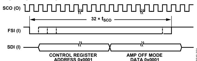
Figure 33. Writing to the AD7765 Control Register Turning Off the On-Board Differential Amplifier
