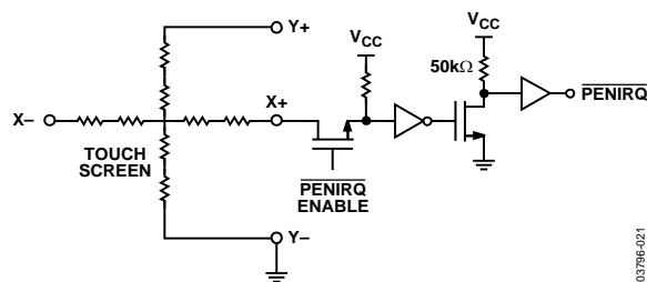
Figure 43. PENIRQ Output Equivalent Circuit
