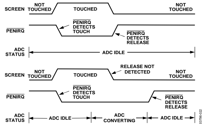
Figure 44. \overline{PENIRQ} Operation for ADC Idle and ADC Converting
