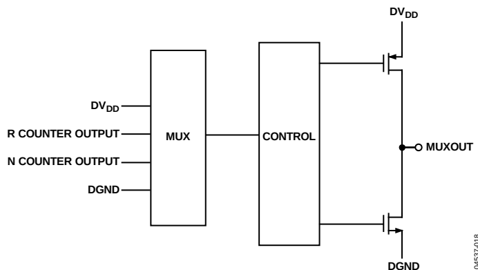
Figure 12. MUXOUT Circuit
