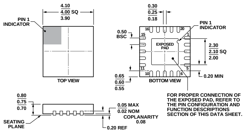
Figure 15. 20-Lead Lead Frame Chip Scale Package [LFCSP_WQ] 4 mm × 4 mm Body, Very Very Thin Quad (CP-20-6)
