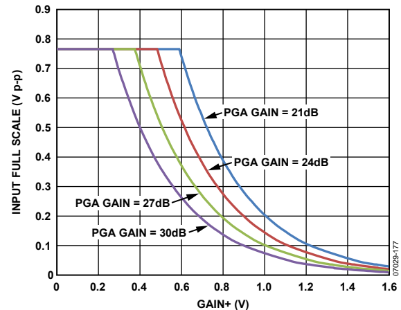
Figure 47. LNA with 15.6 dB Gain Setting/VGA Full-Scale Limitations
