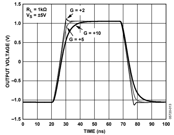
Figure 27. Large Signal Transient Response for Various Gains
