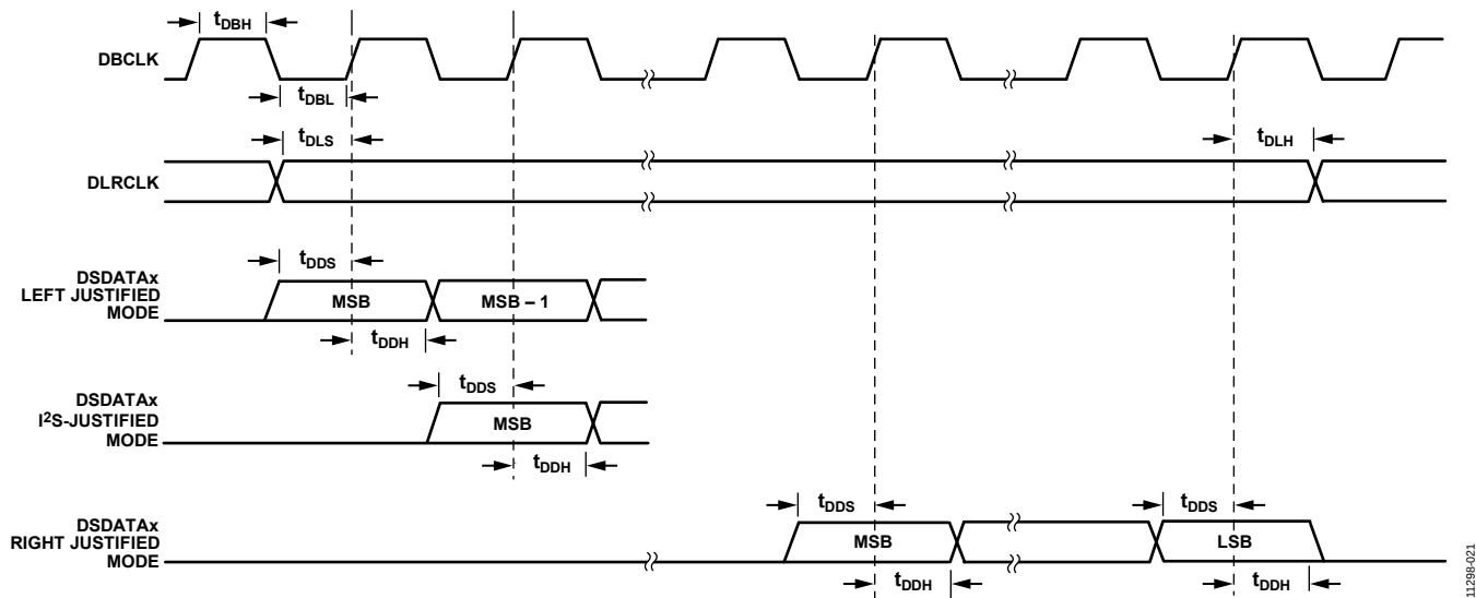
Figure 21. DAC Serial Timing
