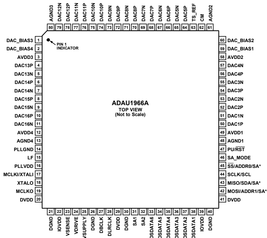
Figure 3. Pin Configuration
