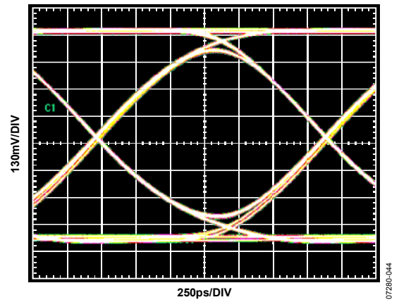
Figure 66. Eye Diagram, 600 Mbps, PRBS31; VH = 2.0 V, VL = 0.0 V
