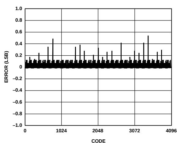
Figure 16. Typical DNL
