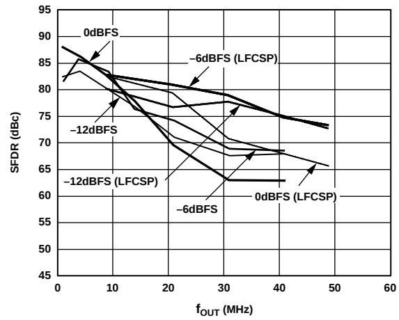
Figure 8. SFDR vs. f_{OUT} @ 165 MSPS
