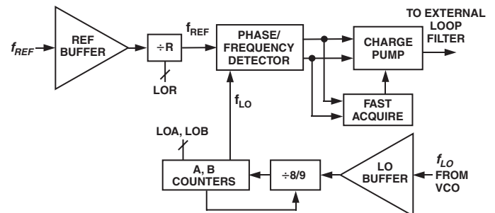
Figure 5. LO Synthesizer
