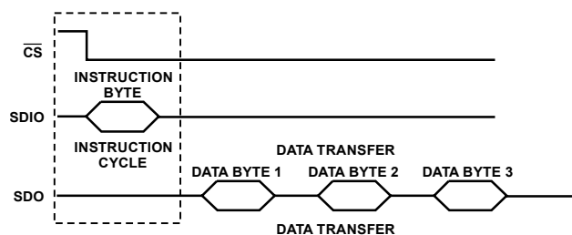
Figure 57. Timing Diagram for Read from AD9854
