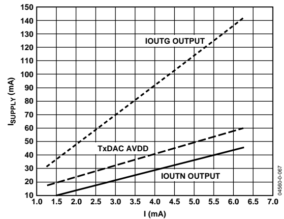
Figure 67. Current Consumption of TxDAC and IAMP in Current-Mode Operation with IOUTN and IOUTG Outputs (Default IAMP Settings)
