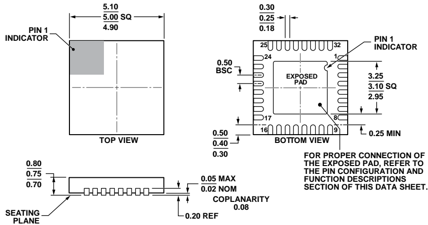
Figure 36. 32-Lead Frame Chip Scale Package [LFCSP] 5 mm × 5 mm Body and 0.75 mm Package Height (CP-32-7)
