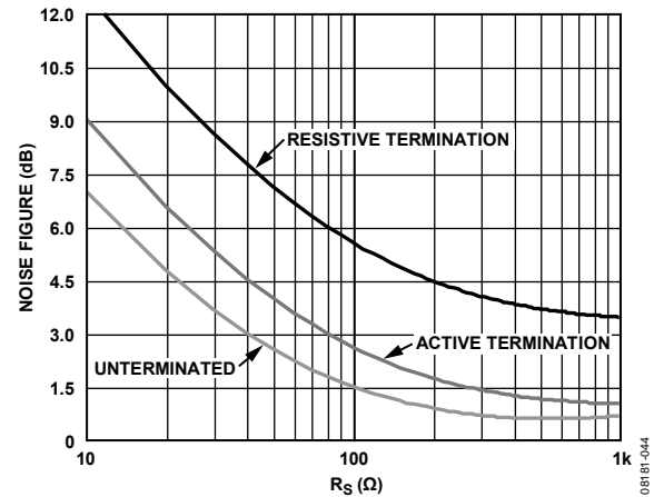
Figure 50. Noise Figure vs. R_S for Resistive Termination, Active Termination Matched, and Unterminated Inputs, V_{\text{GAIN}} = 0.8 \text{ V}
