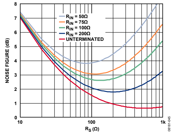
Figure 51. Noise Figure vs. R_S for Various Fixed Values of R_{IN} , Active Termination Matched Inputs, V_{\text{GAIN}} = 0.8 \text{ V}
