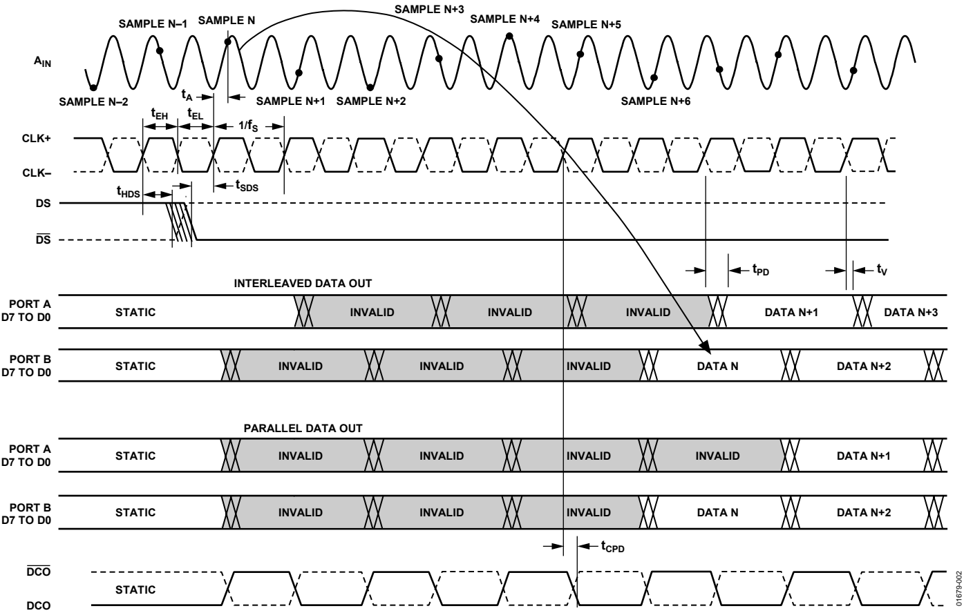
Figure 2. Timing Diagram
