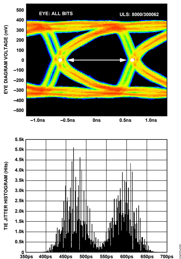
Figure 71. Data Eye for LVDS Outputs in ANSI-644 Mode with Trace Lengths Less than 24 Inches on Standard FR-4 Material, External 100 \Omega Far-End Termination Only
