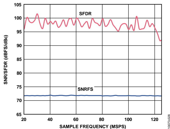
Figure 44. SNR/SFDR vs. Encode, f_{\text{IN}} = 9.7 \text{ MHz} , f_{\text{SAMPLE}} = 125 \text{ MSPS}
